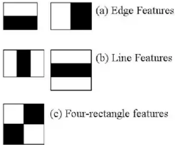
Figure 36: Figure showing types of Haar Features
