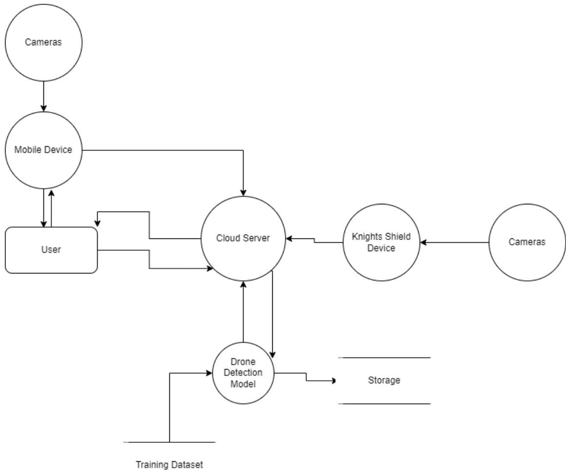
Figure 59: Figure showing the Data Flow Diagram of the Knights Shield System
