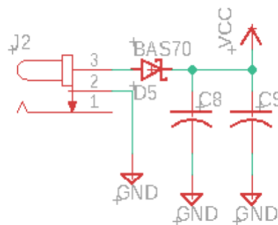
Figure 53: DC Jack Connector
