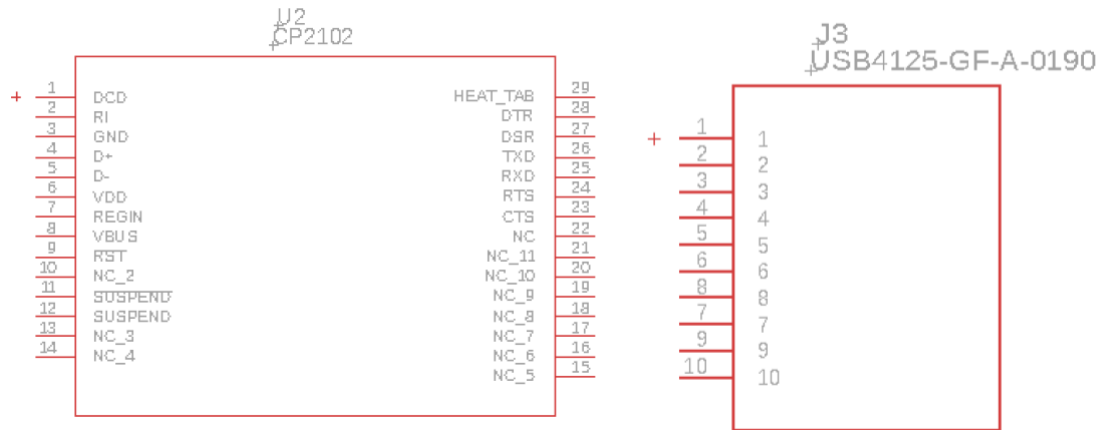
Figure 54: CP2102 USB to UART Bridge and USB-C Receptacle
