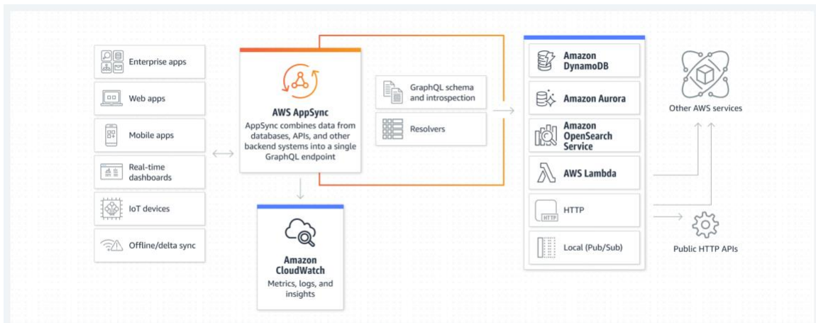
Figure 63: Figure showing feature of AWS AppSync
