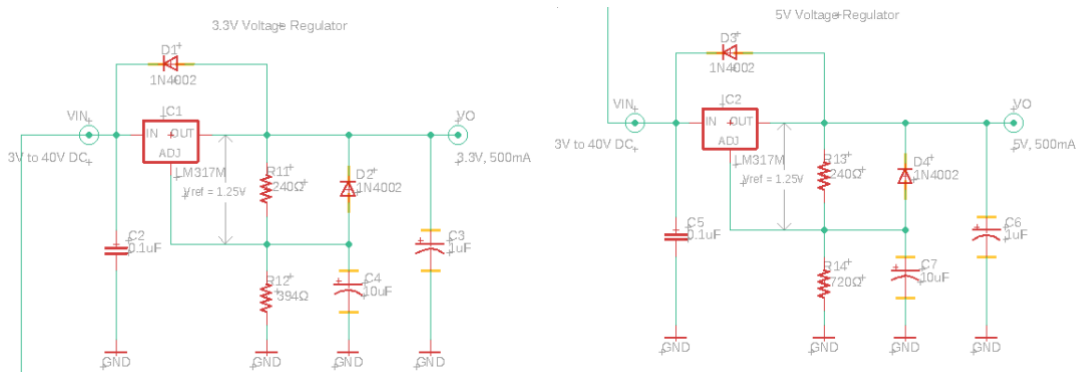
Figure 50: 3.3V and 5V Voltage Regulator
