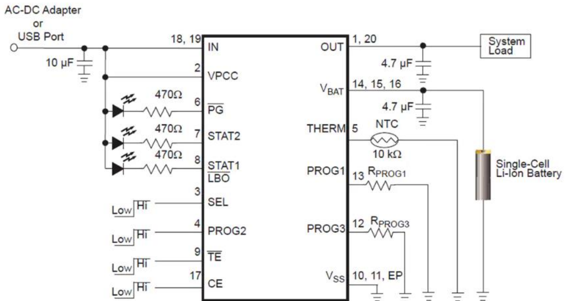
Figure 56: MCP73871 schematic
