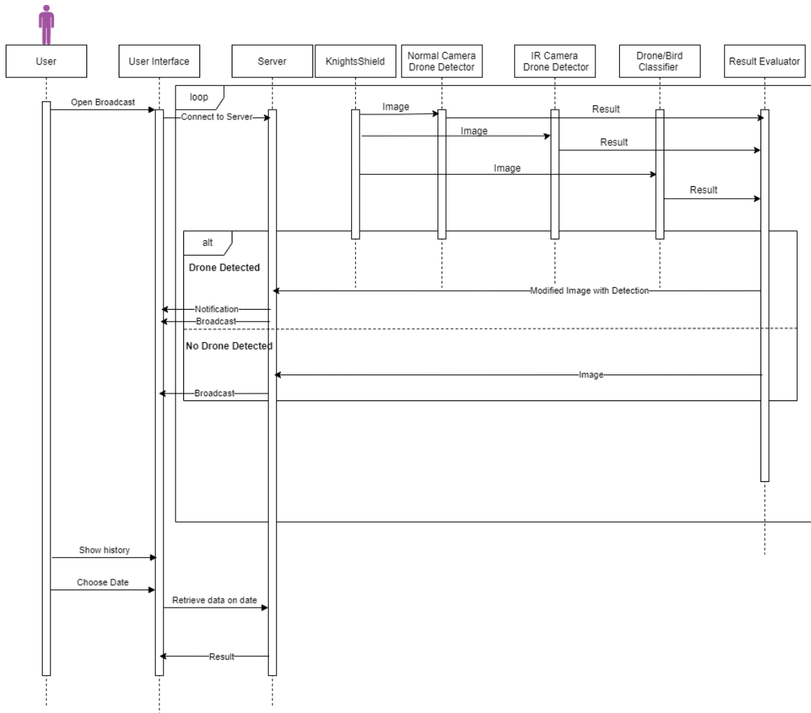
Figure 66: Figure showing the Sequence Diagram of the System
