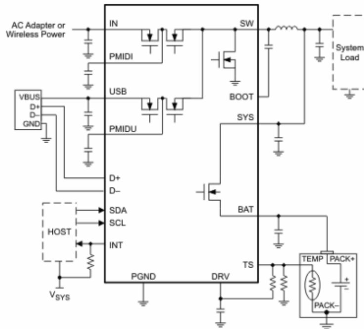
Figure 55: BQ24168 schematic
