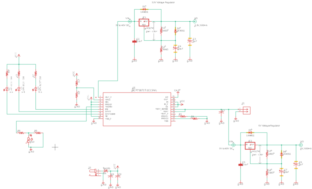
Figure 48: Overall Rough Draft Power System Schematic
