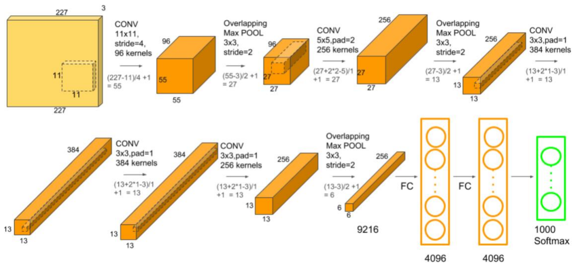
Figure 43: Figure showing the architecture of AlexNet
