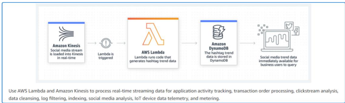
Figure 65: Figure showing feature of Amazon Lambda
