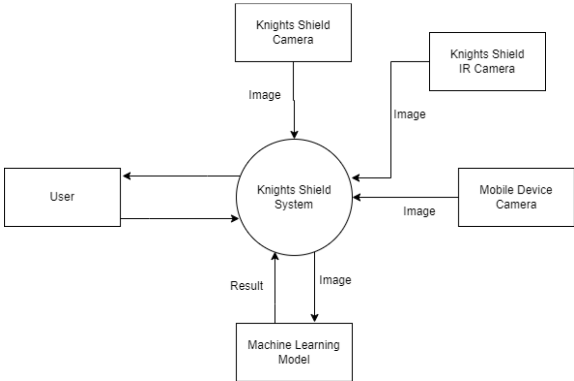
Figure 58: Figure showing the Context Diagram of the Knights Shield System
