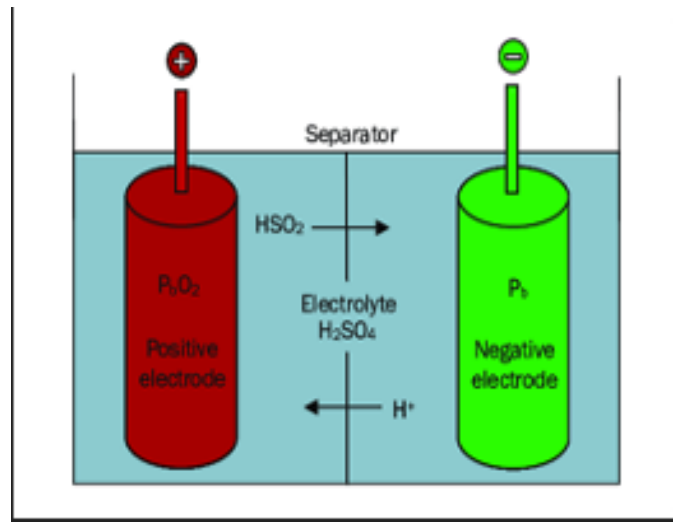
Figure 25: configuration of a lead acid battery
